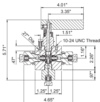
Manual 3-Way Ball Valve
